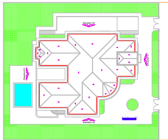
Roof Plan
