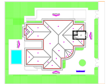
Attic Plan A = 25,31 m 2
