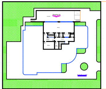
Lower Floor Plan A = 163,94 m 2
