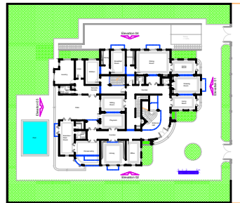
First Floor Plan A = 487,30 m 2
